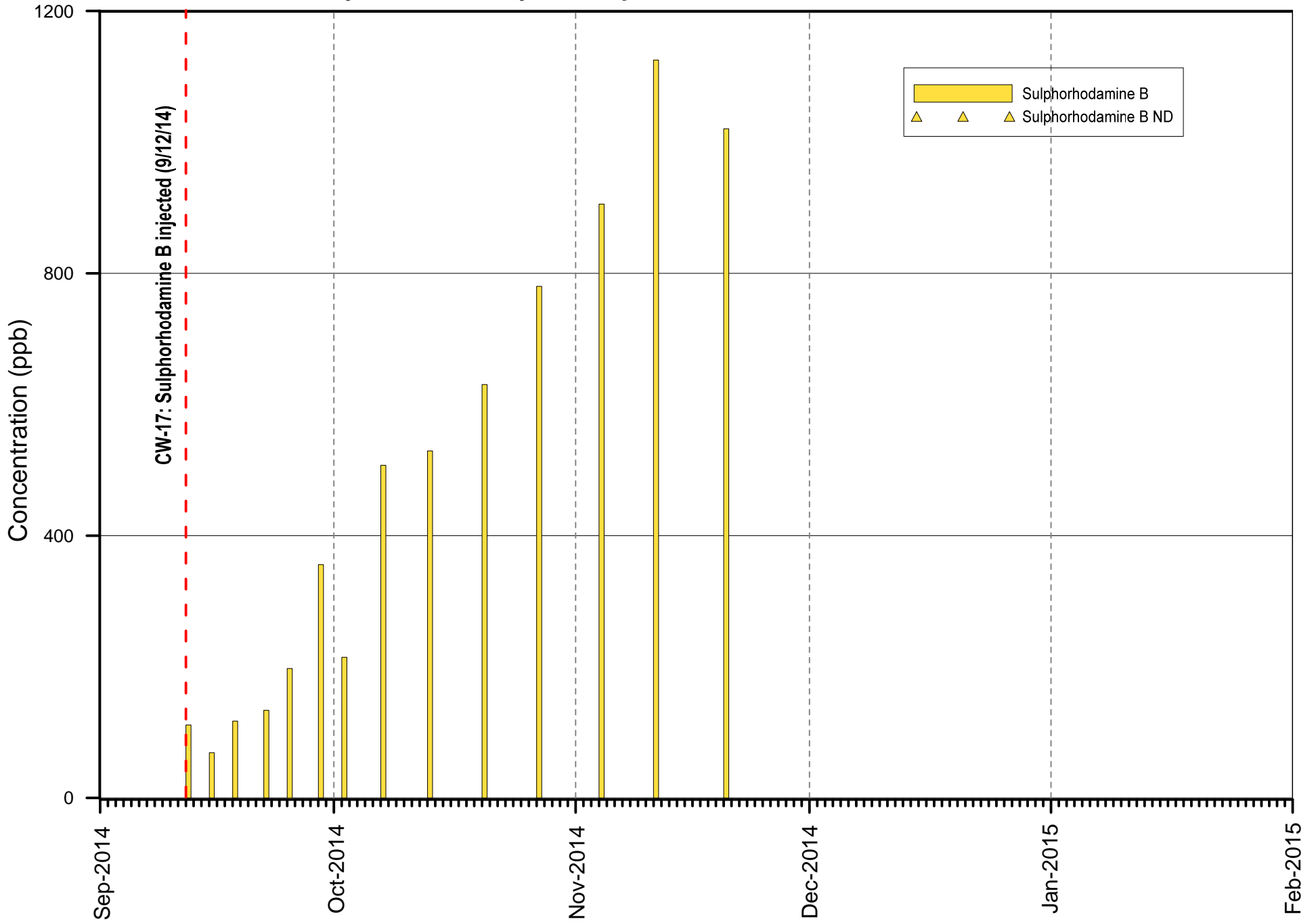
Figure 3.2-8 MW-74S Dye Tracer Analysis Sulphorhodamine B Detections - 2nd Test at CW-17
